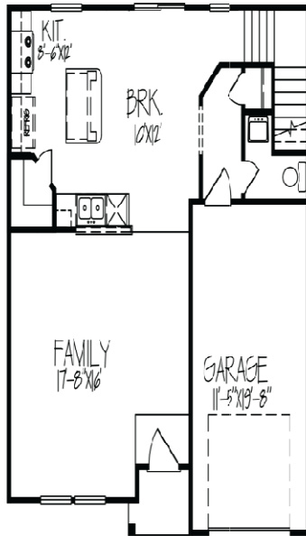
First Floor 1560
