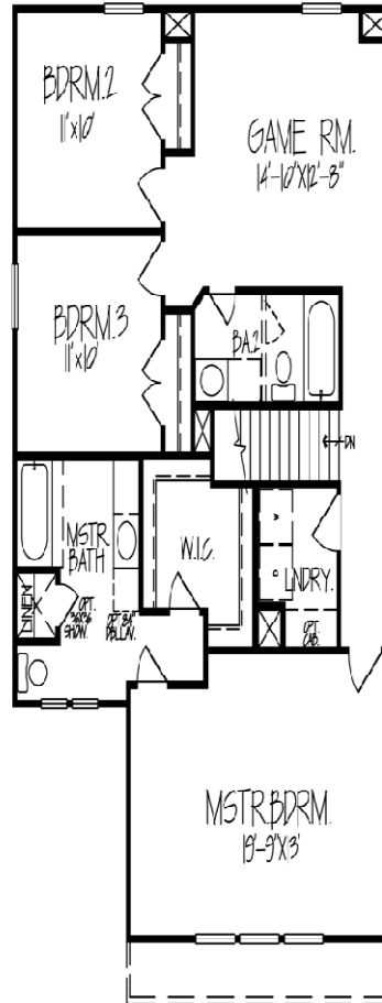
Second Floor 3 Bedroom with Loft
