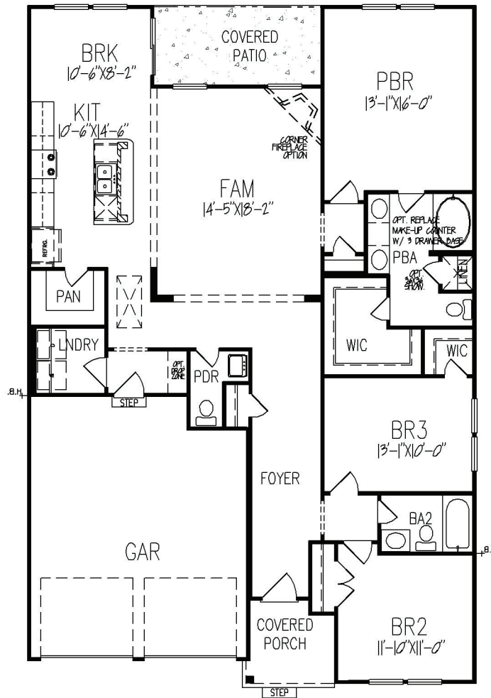
FIRST FLOOR PLAN HEATED AREA - 1,729 Sq.Ft. ROCK HILL PALMETTO - 1731
