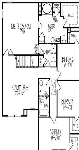
Second Floor 4 Bedroom with Game Room
