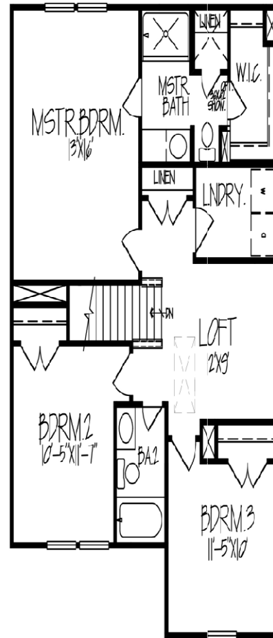
Second Floor 3 Bedroom with Loft
