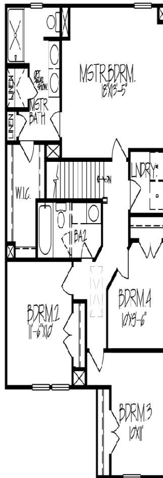
Second Floor 4 Bedroom
