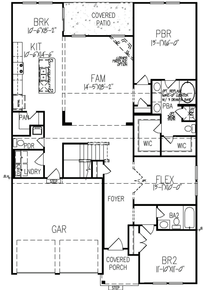
FIRST FLOOR PLAN HEATED AREA - 1,770 Sq.Ft.
