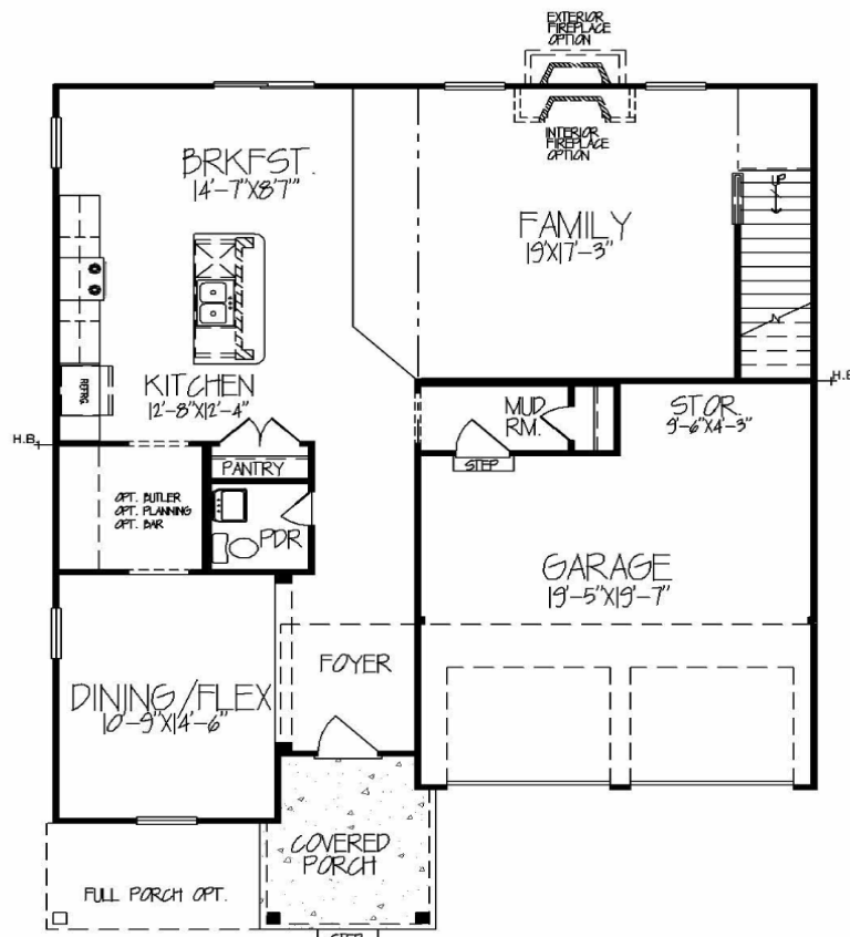
38'-4" X 50'-4" FIRST FLOOR PLAN HEATED AREA = 1,171 S.F. TOTAL HEATED AREA = 2,488 S.F. WILLOW 2367
