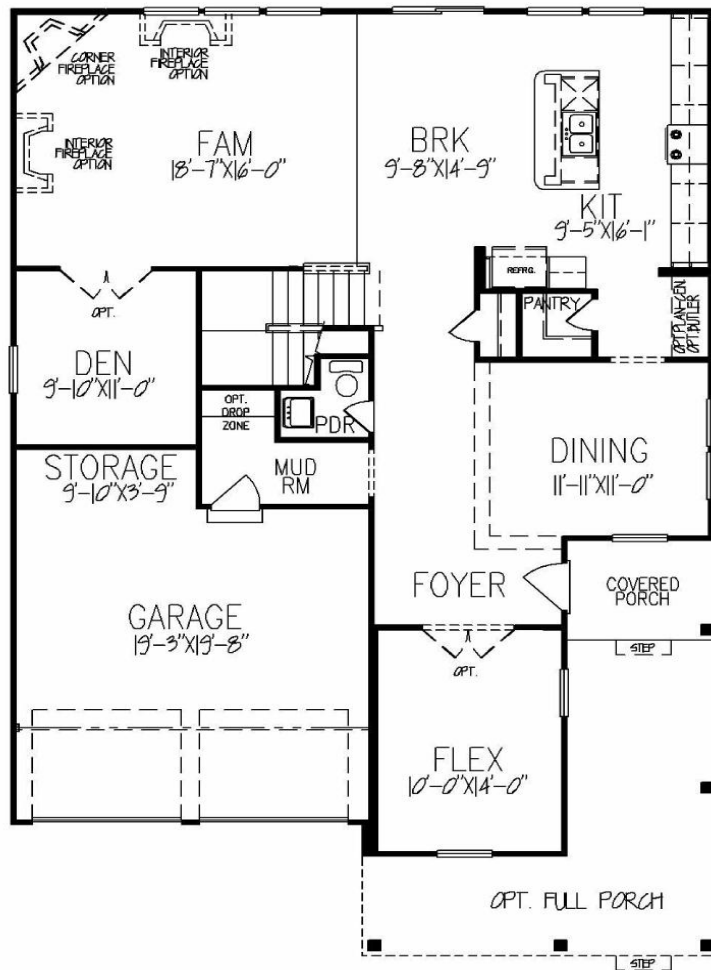
FIRST FLOOR PLAN HEATED AREA = 1,429 HICKORY 3055
